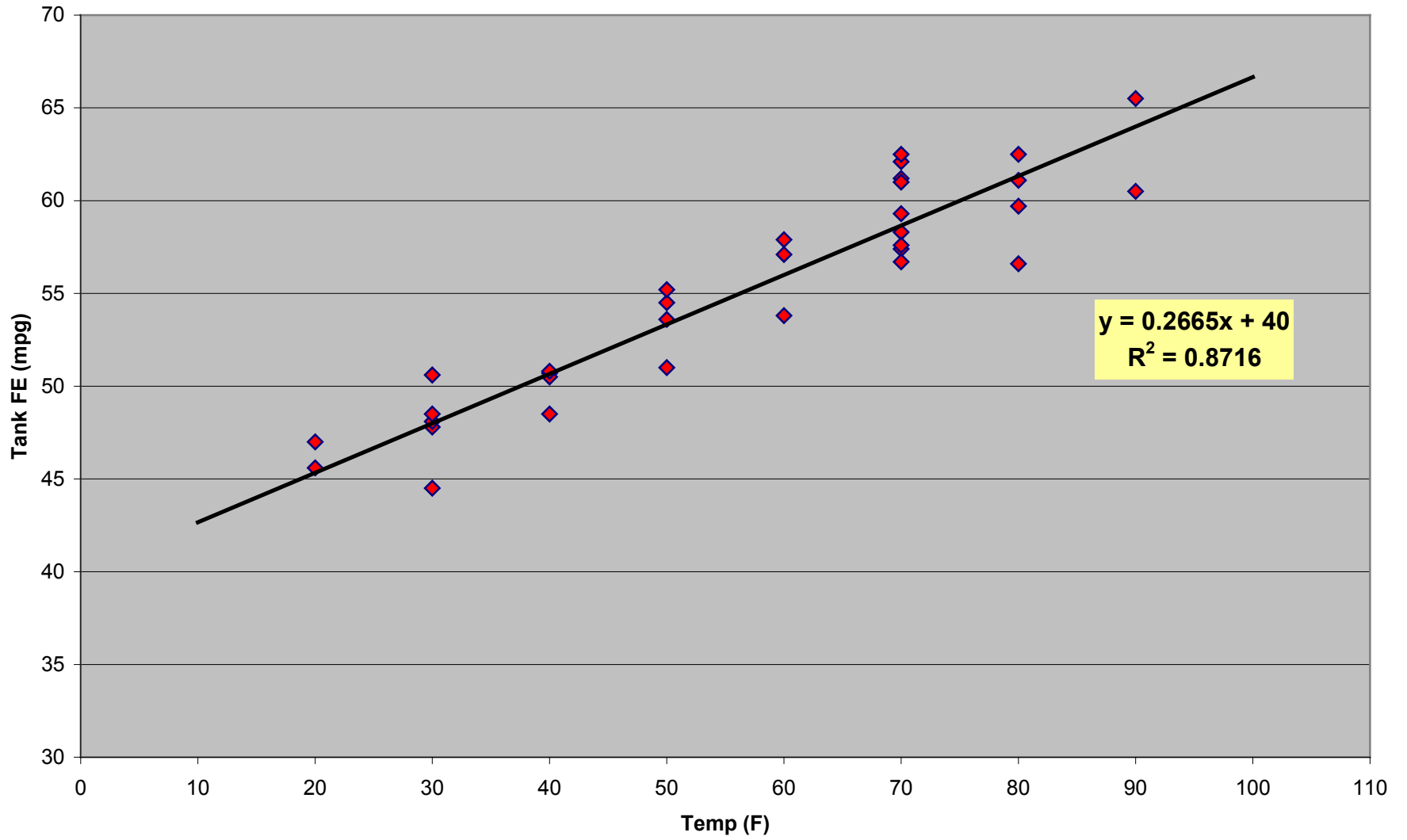
HCH2 - Tank FE vs Outdoor Temp
